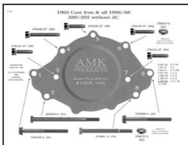
Water Pump Bolt Instructions
